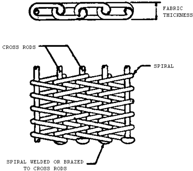
FIGURE 2 METAL MESH CONSTRUCTION
