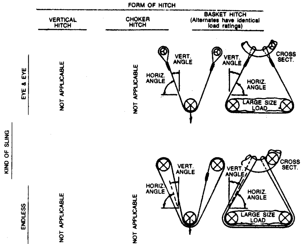
FIGURE 5 SLING CONFIGURATIONS WITH ANGLED LEGS
